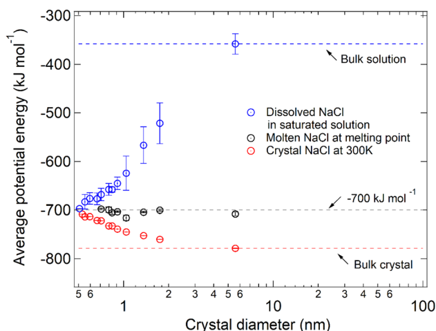
Fig. 4 Average potential energy of NaCl ( \mu_{\text{NaCl}} ) in solution, molten NaCl and crystal. Blue circles represent \mu_{\text{NaCl}} in the saturated droplets at the critical dissolution state. The blue dashed line represents \mu_{\text{NaCl}} in bulk saturated solution ( \approx -358.35 \pm 20.95 \text{ kJ mol}^{-1} ). Black circles represent \mu_{\text{NaCl}} in the molten NaCl at the respective melting points, and the values are all near -700 \text{ kJ mol}^{-1} (grey dashed line). Red circles represent \mu_{\text{NaCl}} in the NaCl crystals at 300 K, and the dashed red line is \mu_{\text{NaCl}} in the bulk NaCl crystal ( \approx -780 \text{ kJ mol}^{-1} ).
