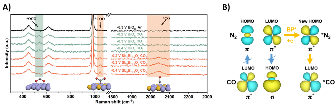
Fig. 20 Mechanistic investigations regarding \text{CO}_2 and \text{N}_2 activation using the \text{Sb}_x\text{Bi}_{1-x}\text{O}_y catalyst. (A) In situ Raman spectra at different potentials. (B) The C–N coupling mechanism regulated by the symmetry matching between the HOMO of \text{*N}_2 and the LUMO of \text{*CO} . Adapted from ref. 203.
