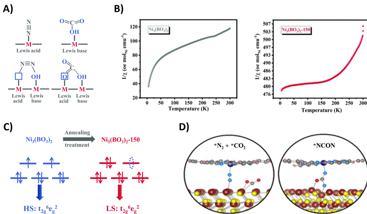
Fig. 21 Mechanistic investigations regarding \text{CO}_2 and \text{N}_2 activation using the \text{Ni}_3(\text{BO}_3)_2\text{-150} (A)–(C) and \text{CoPc-MoS}_2 catalyst (D). (A) Schematic illustration of adsorption of \text{CO}_2 and \text{N}_2 on frustrated Lewis pairs. (B) Temperature-dependent inverse susceptibility 1/\chi plots for pristine \text{Ni}_3(\text{BO}_3)_2 and \text{Ni}_3(\text{BO}_3)_2\text{-150} catalyst. (C) Schematic illustration of the spin-state regulation of \text{Ni}_3(\text{BO}_3)_2 after annealing treatment. (D) Schematic illustration of \text{N}_2 and \text{CO}_2 activation (left) and \text{*NCON} formation (right) on the \text{CoPc-MoS}_2 catalyst. Adapted from ref. 207 (A)–(C) and 205 (D), respectively.
