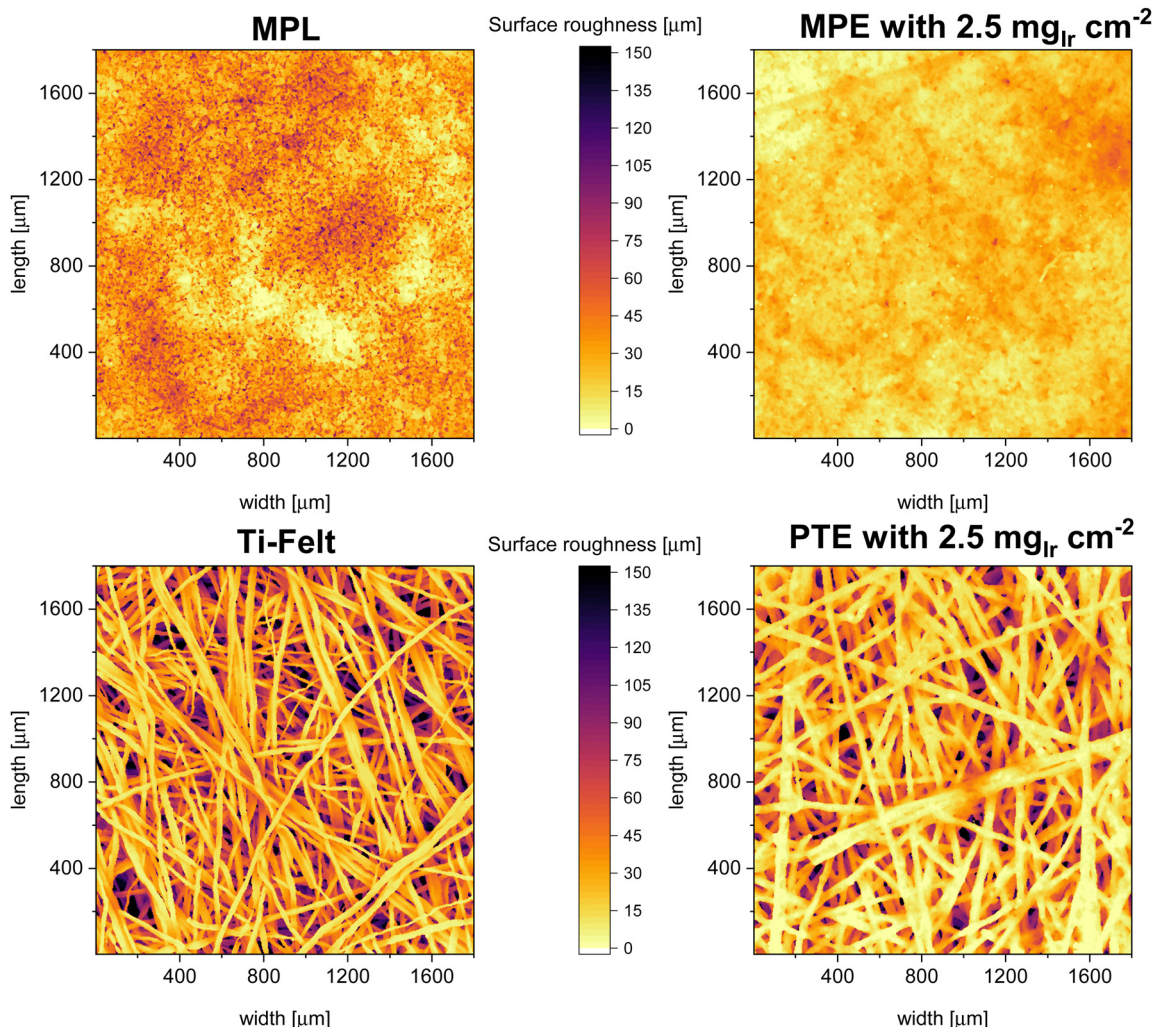
Fig. 5 Surface distance maps from the XTM data of the stand-alone MPL and PTL (Ti-felt) as well as the MPE and PTE with a loading of 2.5 \text{ mg}_r \text{ cm}^{-2} .
