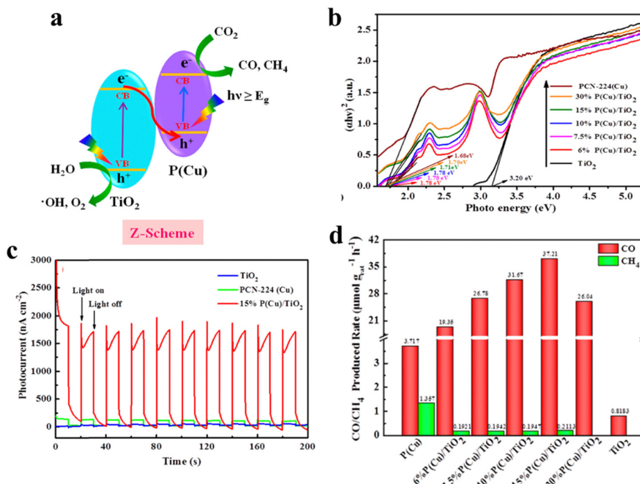
Fig. 14 (a) Direct Z-scheme photocatalytic mechanism. (b) Energy band gaps ( E_g ) of \text{TiO}_2 , \text{PCN-224(Cu)} , and \text{PCN-224(Cu)/TiO}_2 . (c) Photocurrent–time ( I-t ) curves of \text{TiO}_2 , \text{PCN-224(Cu)} , and 15\%\text{P(Cu)/TiO}_2 photoelectrodes at 0.6 V vs. REH bias potential in 0.5 M \text{Na}_2\text{SO}_4 (pH \sim 7.35 ). (d) CO and \text{CH}_4 generation rate over \text{PCN-224(Cu)} , 6\%\text{P(Cu)/TiO}_2 , 7.5\%\text{P(Cu)/TiO}_2 , 10\%\text{P(Cu)/TiO}_2 , 15\%\text{P(Cu)/TiO}_2 , 30\%\text{P(Cu)/TiO}_2 , and \text{TiO}_2 under 300 W Xe lamps. Reproduced from ref. 64. Copyright 2022 ACS.
