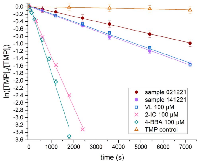
Fig. 2 Degradation of the triplet state probe, TMP, by two aerosol samples (021 221 and 141 221, 10 mg C L -1 ) and three photosensitizers (VL, 2-IC, and 4-BBA). All experiments contained 100 μM TMP. The error bars represent the variation from the theoretical initial TMP concentration.
