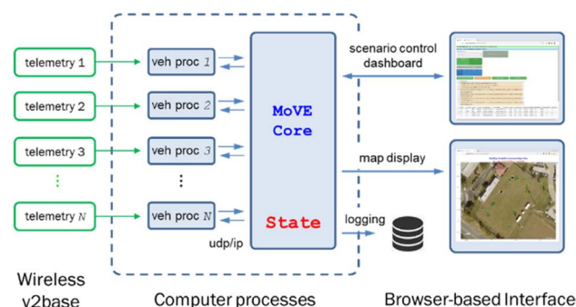
Fig. 3 MoVE architecture with N real vehicles sending telemetry to N vehicle model processes. MoVE Core receives updates from them and user commands before sending state updates to a 2D map, a live updating data table, and logger for post-processing and playback.
