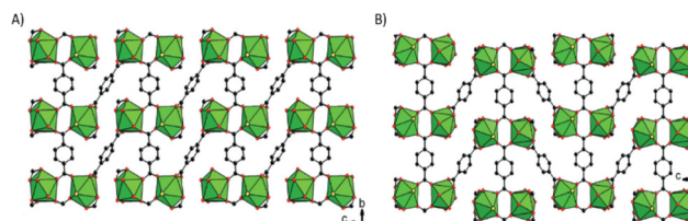
Fig. 11 Connection modes of (A) triclinic (B) monoclinic U 2 Cl 2 (BDC) 3 (DMF) 4 . Dalton Trans. , 44 , 2639–2649, © 2015.
