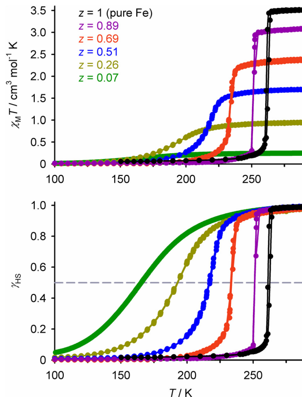
Fig. 2 SCO in different compositions of [\text{Fe}_z\text{Zn}_{1-z}(\text{1-bpp})_2][\text{BF}_4]_2 (Scheme 1). Top, the measured magnetic susceptibility data. Bottom, the same data expressed as the high-spin fraction in the iron content of the samples ( \gamma_{\text{HS}} ). Data points are linked by spline curves for clarity and the dashed line corresponds to \gamma_{\text{HS}} = 0.5 , indicating the SCO midpoint at T_{\frac{1}{2}} . This figure has been adapted from ref. 63 with permission from the Royal Society of Chemistry, copyright 2023.
