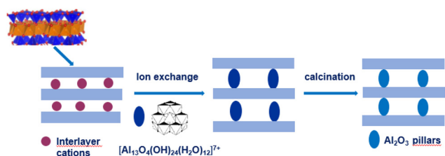
Fig. 1 Preparation of \text{Al}_2\text{O}_3 pillared clays.
