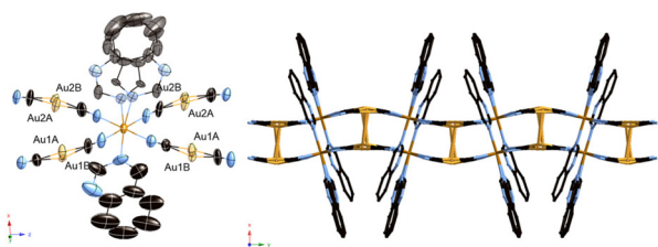
Fig. 1 Crystal structure of complex 1 . (Left: ORTEP structure. Right: packing structure along the X axis.)
