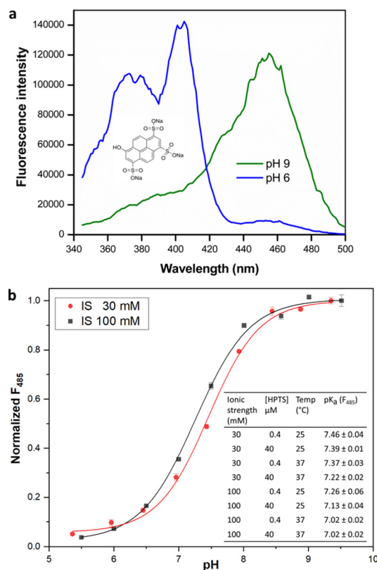
Fig. 1 (a) HPTS structure (inset) and fluorescence excitation spectra, \lambda_{em} = 511 nm. (b) Dependence of fluorescence intensity (485 nm) of HPTS on pH at 25 °C. Inset: pK_a estimates for HPTS under different reaction conditions. Fluorescence measurements were made as described in methods. pK_a values are given as mean \pm SD ( n = 3 ).
