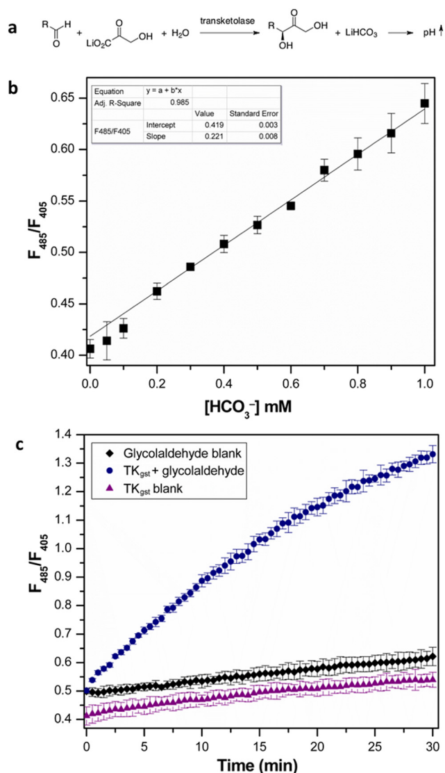
Fig. 2 (a) Transketolase reaction with pH shift. (b) Calibration curve of fluorescence intensity ratio ( I_{\text{ex } 485 \text{ nm}}/I_{\text{ex } 405 \text{ nm}} ) with \text{NaHCO}_3 standard (0–1 mM). All measurements were performed in triplicate. (c) Progress of transketolase reaction with 20 mM glycolaldehyde and 50 mM LiHPA. Error bars represent SD from triplicate measurements.
