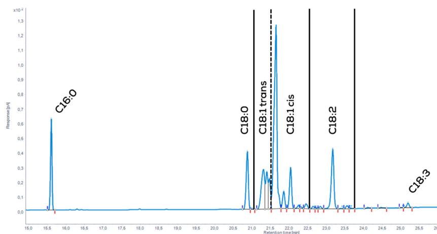
Fig. 6 Typical chromatogram of a partially hydrogenated soybean oil derived methyl ester analyzed by GC-FID. Separation on a 90 m DB FastFAME column. Methylation by addition of 50% (w/w) TMSH in methanol.
