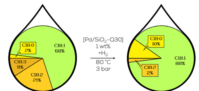
Fig. 21 C18 fatty acid composition in the hydrogenation of canola oil-derived biodiesel over macroporous Pd on SiO 2 as performed by Luengnaruemitchai. 127
