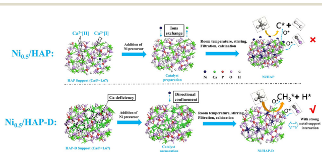
Fig. 7 Schematic diagram of catalyst synthesis path and DRM reaction route. Reproduced from ref. 12 with permission from Fuel, copyright 2022.
