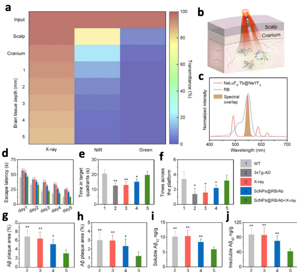
Fig. 20 (a) Transmittance of X-ray, NIR and green light through the scalp, cranium and different thicknesses of brain tissue. (b) Schematic illustration for the X-ray activated photodynamic therapy for Alzheimer's disease by inhibiting A \beta aggregation in the brain. (c) Spectral overlap between X-ray activated luminescence from NaLuF 4 :Tb 3+ and the absorption spectrum of Rose Bengal. In vivo comparison of (d) escape latency, (e) time in target quadrants and (f) times across the platform of Alzheimer's disease mice in the Morris water maze test. Quantification of A \beta plaques in the (g) cortex and (h) hippocampus, as well as (i) soluble and (j) insoluble A \beta 42 levels in the brain after different treatments. Reproduced with permission from ref. 14. Copyright 2023, Elsevier.
