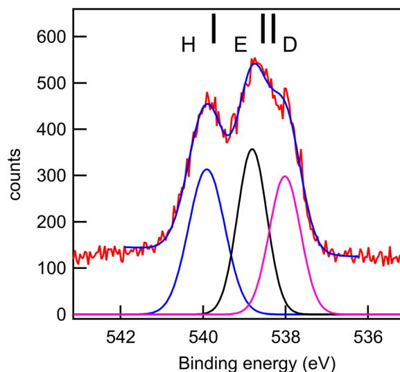
Fig. 11 O 1s core-level spectrum (red line: data; blue line: smoothed data) of fenopropfen and a fit with three Gaussian functions, whose integrated intensity variations were limited to \pm 10\% of the mean intensity, and whose energies and widths were allowed to vary freely. Photon energy: 628 eV. Black bars: theoretical vertical ionization potentials (at the SAC-CI/MIDI! level of calculation).
