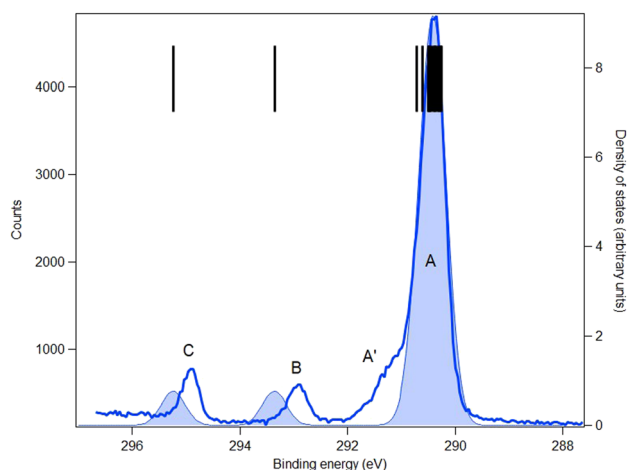
Fig. 9 C 1s core-level spectrum (blue line) and simulation (blue full area) of ketopropfen. Photon energy: 382 eV. Black bars: theoretical vertical ionization potentials (at the SAC-CI/MIDI! level of calculation).
