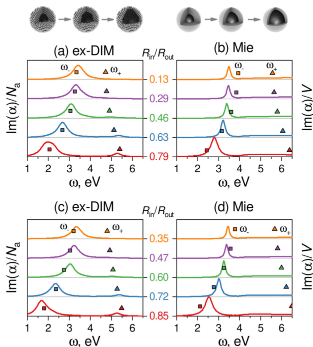
Fig. 11 Normalized imaginary polarizability from the Ex-DIM model (left) and Mie theory (right) calculations for nano-shells with fixed outer radius R_{\text{out}} : 5.97 nm (top) and 7.94 nm (bottom). Squares and triangles give the positions of the symmetric ( \omega_- ) and anti-symmetric ( \omega_+ ) modes from eqn (1) in ref. 143 with \omega_B = 5.78 eV (Ex-DIM) and \omega_B = 6.82 eV (Mie). From ref. 143.
