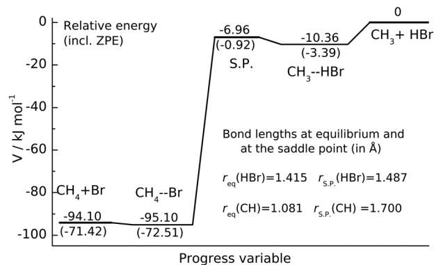
Fig. 1 Potential energy profile of \text{CH}_3 + \text{HBr} reaction. The energy levels of the stationary points characterizing the Czako–Góger–Szabó–Lendvai PES 13 are given in kJ mol -1 . The zero-point energy corrected energies are shown in parentheses. The S.P. denotes the saddle point.
