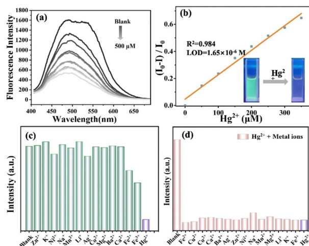
Fig. 2 (a) The fluorescence emission spectrum of DvDf-C3XJ-COF dispersed in EtOH:H 2 O = 1:1 with the addition of different amounts of Hg 2+ (0 to 500 \mu M). (b) The linear relationship between the fluorescence intensity of DvDf-C3XJ-COF with the concentration of Hg 2+ (Inset: A photograph demonstrating the fluorescence change of DvDf-C3XJ-COF in EtOH:H 2 O = 1:1 following the addition of 300 \mu M Hg 2+ , illuminated under a UV lamp with \lambda_{\text{ex}} = 365 nm). (c) The fluorescence intensity ratio of DvDf-C3XJ-COF in the presence of different metal ions (300 \mu M). (d) The fluorescence intensity ratio of DvDf-C3XJ-COF + Hg 2+ in the presence of different metal ions (300 \mu M).
