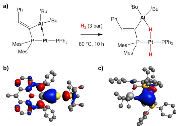
Fig. 5 (a) Experimentally reported reactivity of a Pt \rightarrow Al complex with \text{H}_2 . 52 (b) and (c) Isosurfaces of the HOMO of the gold-alumanyl complex (b) and platinum-alumanyl complex (c). The isovalue is 3 m_e a_0^{-3} . The isosurfaces have been taken and adapted with permission from ref. 50. Copyright 2023, Royal Society of Chemistry.
