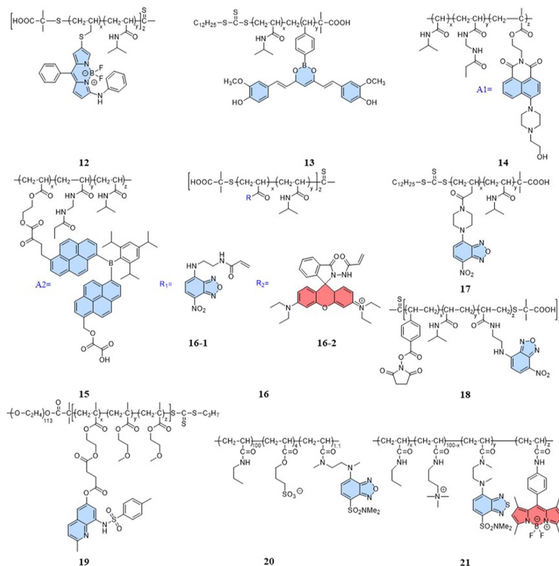
Fig. 4 Structures of polarity-sensitivity-based temperature probes.
