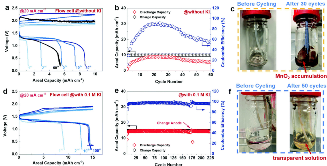
Fig. 13 The GCD performance of Zn/Mn RFB recorded at 20 \text{ mA cm}^{-2} (a)–(c) without KI and (d)–(f) with 0.1 M KI (reproduced from ref. 82 with permission from The Royal Society of Chemistry).
