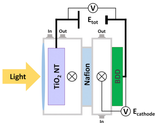
Fig. 3 Schematic diagram of the photoelectrochemical cell. The symbol \otimes represents the reference electrode: \text{Ag}/\text{AgCl} , \text{KCl} (sat'd). E_{\text{cathode}} means that the potential at the BDD cathode is fixed with respect to the reference electrode. E_{\text{tot}} means that the potential is fixed between the BDD and \text{TiO}_2 NT electrodes. The reference electrode in the \text{TiO}_2 NT electrode compartment is used to monitor the potential at \text{TiO}_2 NTs. Black lines are cable connections. In and Out are connecting tubes for electrolyte circulation. A quartz window permits the light to reach the \text{TiO}_2 NT photoanode.
