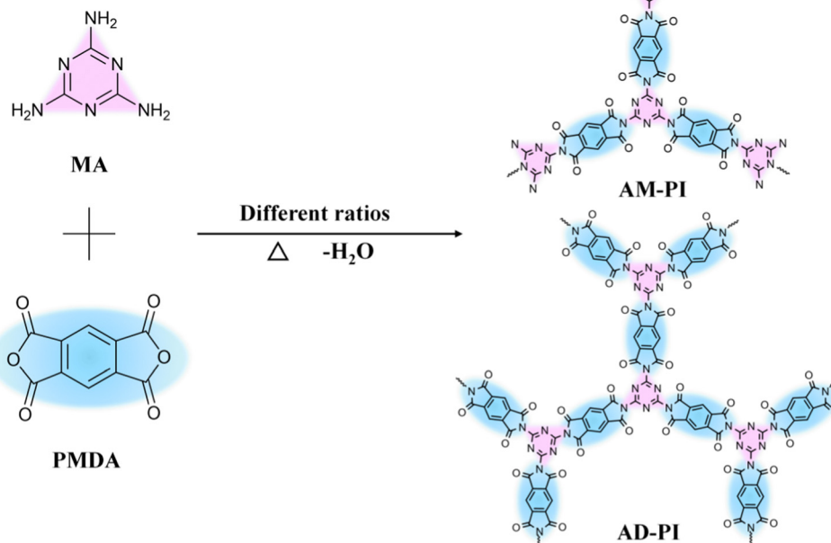
Scheme 1 Reaction scheme for the synthesis of AM-PI and AD-PI .
