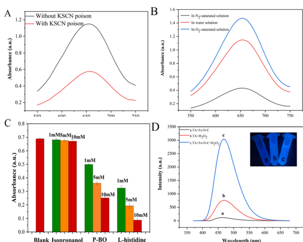
Fig. 7 (A) The absorbance changes of ox-TMB poisoned with 10 mM KSCN in HAC–NaAc buffer (pH = 4). (B) UV absorbance spectra of the colorimetric reaction in a saturated N_2/O_2 atmosphere. (C) Absorbances after inhibition of the reaction by different scavengers. (D) The effect of the Fe–N–C on the formation of the hydroxyl radical with TA as a fluorescence probe.
