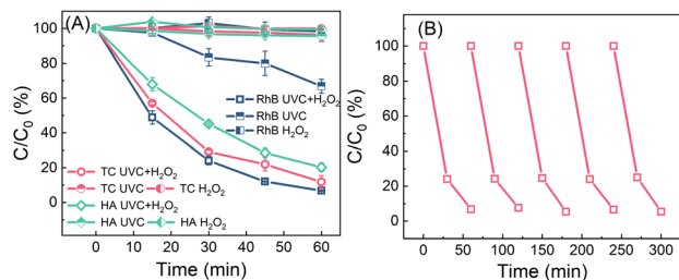
Fig. 4 (A) The removal of RhB, TC and HA via UVC/H 2 O 2 , UVC and H 2 O 2 processes in batch tests; and (B) recyclability of the process for RhB removal (RhB, HA or TC: 1 mg L -1 ; H 2 O 2 : 10 μM).
