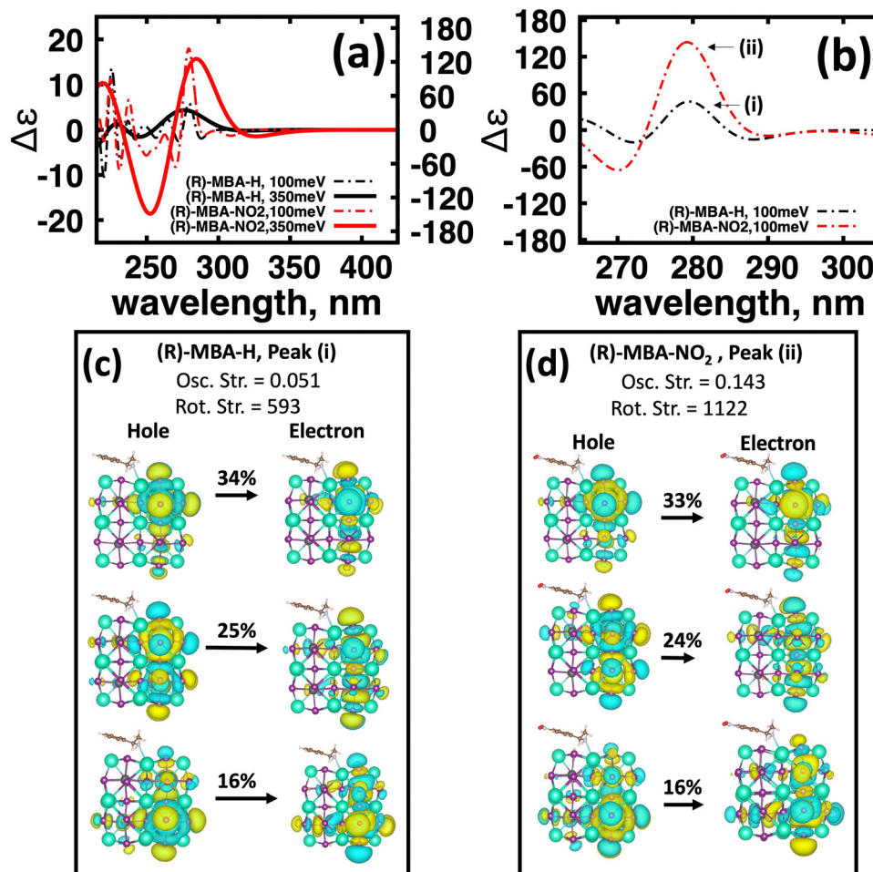
Fig. 4 Functionalization of ( R )-MBA-H with NO 2 to facilitate chirality transfer. (a) Comparison of ( R )-MBA-H (black) and ( R )-MBA-NO 2 (red) with 350 meV (solid) and 100 meV (dash-dot) broadenings. (b) Circular dichroism peaks of the first CD band labeled peak (i) for ( R )-MBA-H and (ii) for ( R )-MBA-NO 2 . (c) Natural transition orbitals of ( R )-MBA-H for peak (i) with corresponding oscillator and rotatory strengths. (d) Natural transition orbitals of ( R )-MBA-NO 2 for peak (ii) with corresponding oscillator and rotatory strengths.
