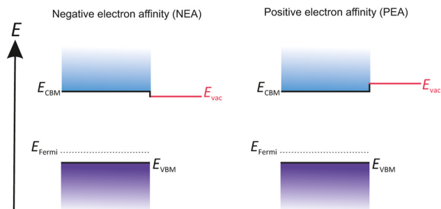
Fig. 4 Comparative illustration of the difference between PEA and NEA surfaces regarding the location of the E_{\text{vac}} .
