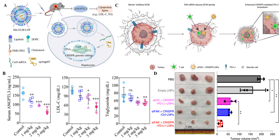
Fig. 3 Therapeutic gene editing through LNP-based targeted delivery of CRISPR/Cas9 in mice to drive loss-of-function mutations in Angptl3 to reduce lipid levels in the blood. (B) Serum ANGPTL3, LDL, and triglyceride levels in mice after 100 of LNP-CRISPR delivery. Adapted from (Qiu et al. 2021). 80 Copyright (2021) National Academy of Sciences. (C) Schematic of addressing tumor mechanics to unlock a double-checkpoint cancer blockage to promote cancer therapy. (D) The excised tumor volume shows modified LNP-CRISPR's in vivo therapeutic efficiency. Reproduced with permission from (Zhang et al. 2022). 93
