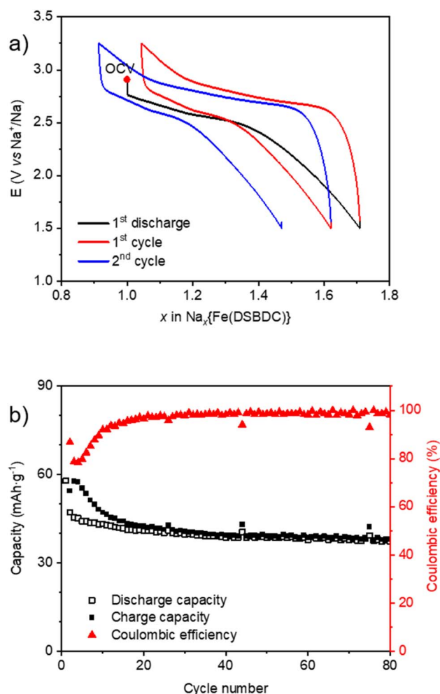
Fig. 8 Electrochemical behaviour of \text{Na}\{\text{Fe}(\text{DSBDC})\} in a half-cell vs. Na cycled in the voltage range of 1.5–3.25 V vs. \text{Na}^+/\text{Na} ( 1\text{ e}^- exchanged per Fe in 10 h). (a) Potential vs. a number of inserted/extracted \text{Na}^+ in the first two cycles. (b) Corresponding capacity retention and coulombic efficiency curves upon long-term cycling.
