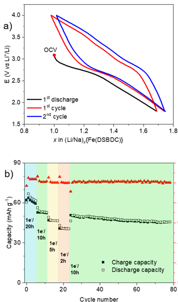
Fig. 7 Electrochemical behaviour of \text{Na}\{\text{Fe}(\text{DSBDC})\} measured in a half-cell vs. Li cycled in the voltage range of 1.8–4.0 V vs. \text{Li}^+/\text{Li} . (a) Potential composition trace for the first two cycles at 1\text{ e}^- exchanged per Fe in 20 h (OCV = open circuit voltage); (b) rate capability cycling test and corresponding coulombic efficiency trace.
