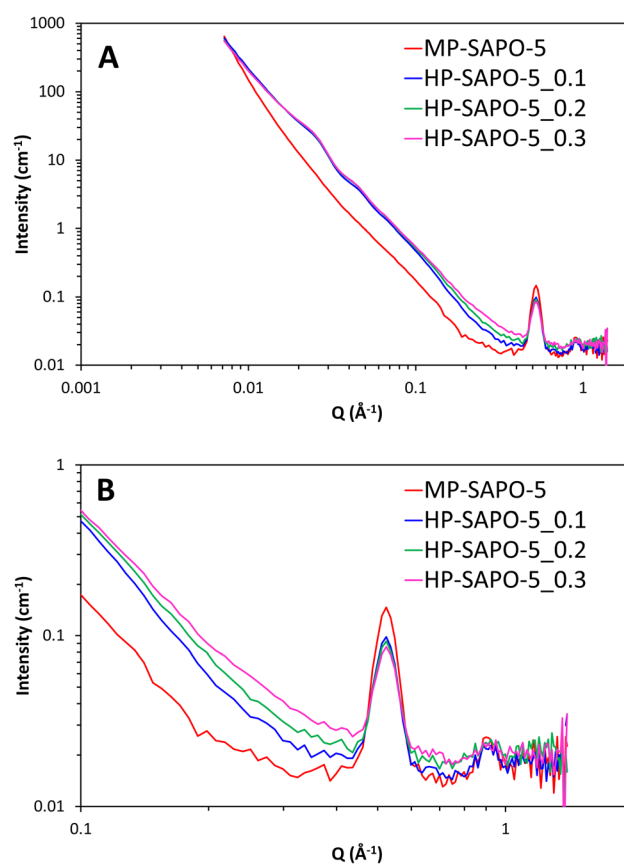
Fig. 6 SANS data of the four dried, bare, SAPO-5 species over full Q range (A) and zoomed in on high Q range (B).
