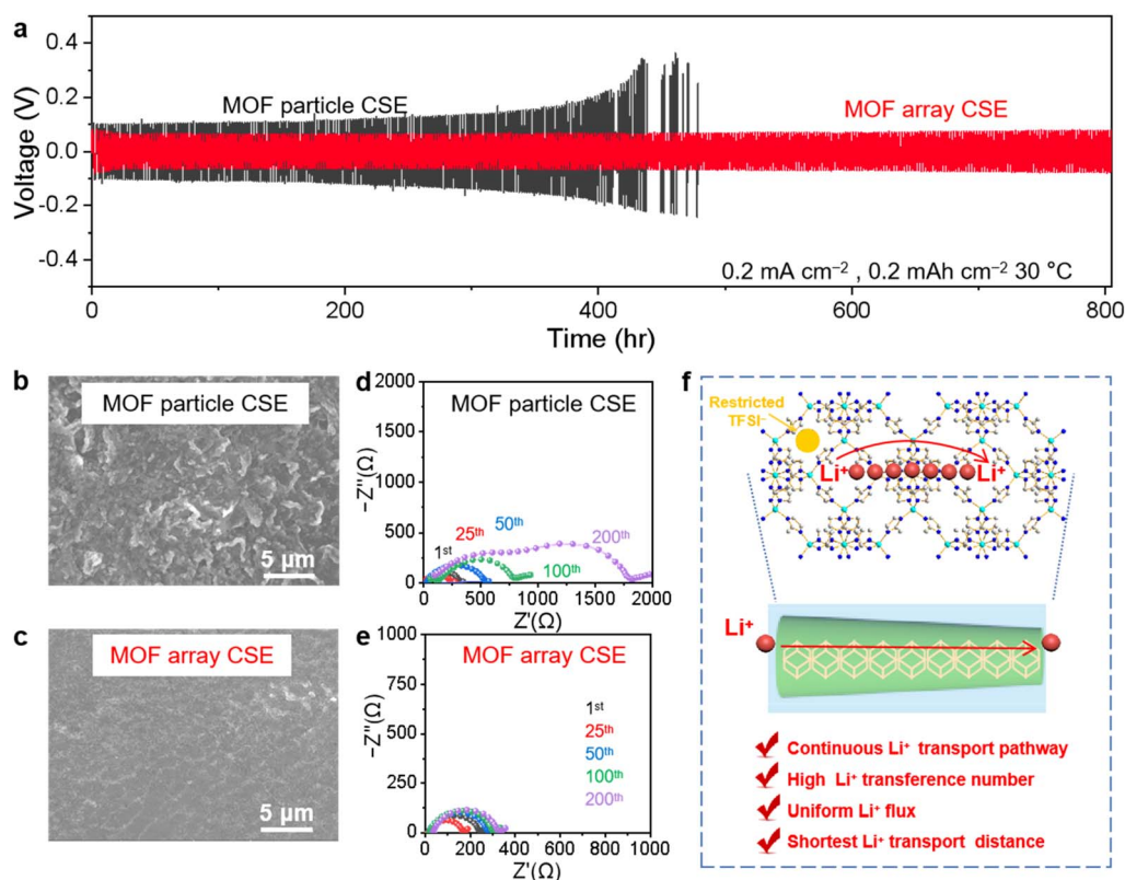
Fig. 4 Li plating/stripping stability. (a) Long-term cycling stability of symmetric Li||Li cells at a current density of 0.2 \text{ mA cm}^{-2} for 0.2 \text{ mA h cm}^{-2} at 30^\circ\text{C} . SEM images of Li-metal recovered from symmetric Li||Li cells using (b) the MOF particle CSE and (c) MOF array CSE after 200 cycles. Electrochemical impedance spectra of symmetric Li||Li cells using (d) the MOF particle CSE and (e) MOF array CSE after different number of cycles at 30^\circ\text{C} . (f) Schematic illustration of the ion transport behavior with a MOF array CSE, where the MOF array offers a continuous and rapid ion transport pathway with the shortest distance, leading to a homogeneous \text{Li}^+ flux and high \text{Li}^+ transference number.
