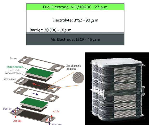
Fig. 16 Sunfire solid oxide cell and stack technology for co-SOE electrolysis (Masini et al., 2019; Sunfire, 2022). 69,70
