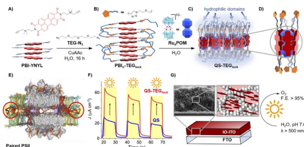
Fig. 18 Second-generation quasomes, exploiting an inter-locked multi-chromophoric antenna system based on PBI photosensitizers bearing hydrophilic tetraethylene glycol chains (TEG). Reprinted from ref. 39 with permission from the American Chemical Society, copyright 2022.
