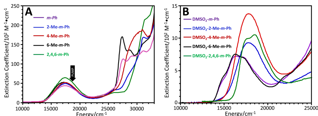
Fig. 3 (A) Electronic absorption spectra of (bpy)Pt(CAT-B-NN) complexes (shown in Fig. 1A) as solutions in CH 2 Cl 2 at 298 K. (B) Electronic absorption spectra of (DMSO) 2 Pt(CAT-B-NN) complexes (shown in Fig. 1C) as solutions in CH 2 Cl 2 at 298 K.
