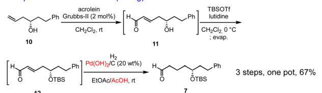
Scheme 3 Four-pot reaction from 9 to 7 and one-pot reaction from 10 to 7 .
