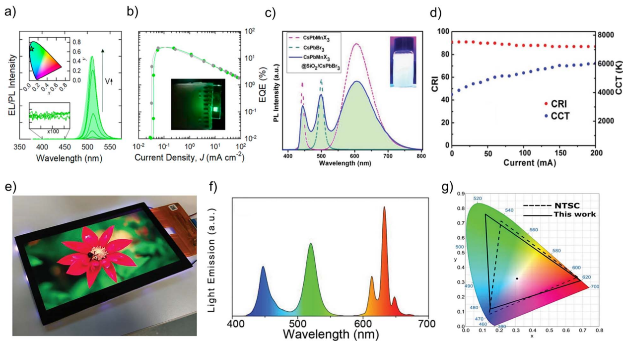
Fig. 4 (a) EL spectra and (b) EQE of ultrabright green-LEDs using PeNCs: \text{NiO}_x composites as active layers. Reproduced under the terms of the CC-BY license. 71 Copyright 2023, The Authors. American Chemical Society. (c) Typical PL spectra of individual \text{CsPbBr}_3 (sea-green curve), \text{CsPbMnX}_3 @ \text{SiO}_2 (pink curve), and nanocrystal combination (blue curve) under UV illumination. The inset of Fig. 4c shows the white-light emission produced by the \text{CsPbBr}_3 + \text{CsPbMnX}_3 @ \text{SiO}_2 PeNC mixture. (d) CRI and CCT of a WLED device fabricated from the nanocrystal combination as a function of diverse driving currents during device operation. Reproduced with permission. 73 Copyright 2019, John Wiley & Sons, Inc. (e) Fabricated LCD display with its corresponding (f) PL spectrum and (g) estimated CIE color coordinates for white color emission produced by the LCD prototype (black line) compared with the NTSC standard color gamut area of CIE1931 (dashed line). Reproduced under the terms of the CC-BY license. 74 Copyright 2022, The Authors. John Wiley & Sons, Inc.
