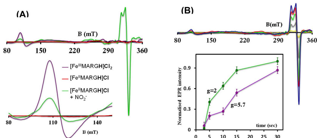
Fig. 4 (A) X-band EPR spectra of [\text{Fe}^{\text{III}}]\text{MARGH}]\text{Cl}_2 (violet) and [\text{Fe}^{\text{II}}]\text{MARGH}]\text{Cl} (red). The green spectra correspond to the \{\text{FeNO}\}^7 species and the ferric porphyrin generated in the reaction of [\text{Fe}^{\text{II}}]\text{MARGH}]\text{Cl} with [\text{NBu}_4]\text{NO}_2 . (B) The corresponding spectra in different time intervals upon addition of [\text{NBu}_4]\text{NO}_2 to [\text{Fe}^{\text{II}}]\text{MARGH}]\text{Cl} and a plot of normalized EPR intensities of the axial (violet) and rhombic (green) signals with time.
