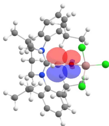
Furthermore, the NBO analysis shows a significant electron donation from the LP orbital (which denotes a lone pair orbital) of oxygen to the vacant p orbital of boron in 2 , with a stabilization energy of 85.4 kcal mol -1 (see Fig. 4). This indicates
