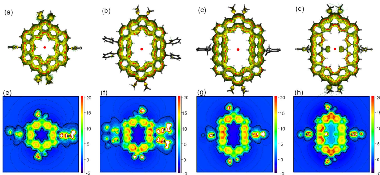
Fig. 4 Calculated ACID plots (contribution from \pi -electrons only) of (a) K1 , (b) K2 , (c) K3 , and (d) K3-R . The magnetic field is perpendicular to the XY plane and points out through the paper. The red arrows indicate the clockwise (diamagnetic) current flow. Calculated 2D ICSS zz maps for (e) K1 , (f) K2 , (g) K3 , and (h) K3-R .
