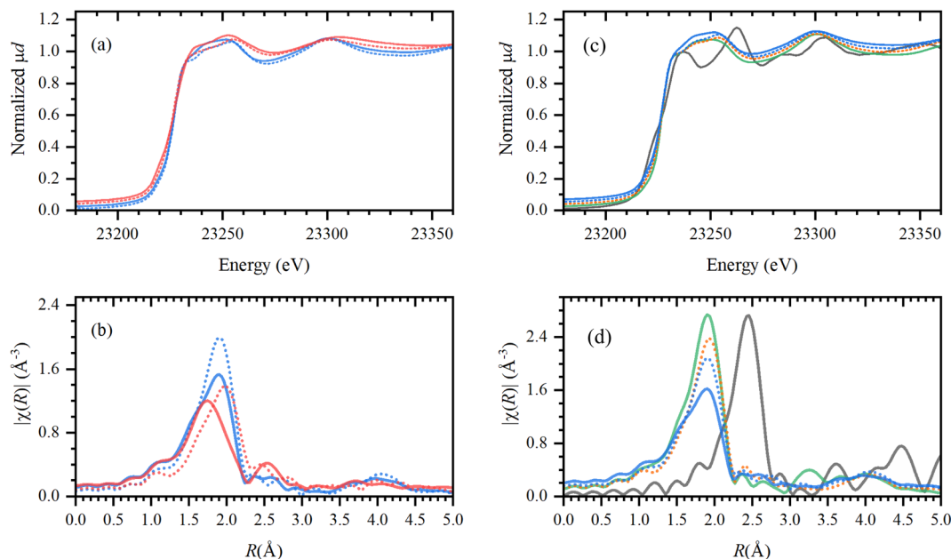
Fig. 10 Left: XANES (a) and phase-uncorrected FT-EXAFS (b) data for the active Rh catalyst (H(CO)Rh(PPh 3 ) 3 ) trapped in Bu 4 PfCl (blue) and Bu 4 PfBr (red); characterized before (solid line) and after reaction (dashed line) with PVC. Right: XANES (c) and phase-uncorrected FT-EXAFS (d) data for the Rh catalyst in Bu 4 PfCl (blue, solid and dashed, before and after reaction), and comparison to RhCl 3 in Bu 4 PfCl after reaction with PVC (orange); reference compounds RhCl 3 (green) and Rh-foil (gray). Detailed descriptions of the samples can be found in the ESI, Table S1.†
