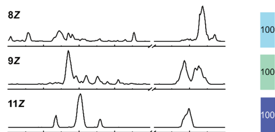
Synthetic mixtures: composite spectra
