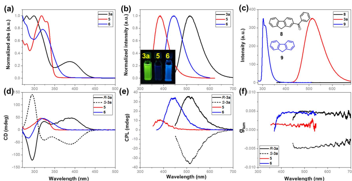
Fig. 2 (a) UV-vis and (b) fluorescence spectra of 3a , 5 , and 6 in CH 3 CN; (c) fluorescence spectra of 3a ( 2 \times 10^{-5} M), 8 ( 2 \times 10^{-5} M), and 9 ( 5 \times 10^{-6} M) in CH 3 CN; (d) ECD and (e) CPL spectra of P - 3a , M - 3a , 5 , and 6 in CH 3 CN ( 5 \times 10^{-5} M); (f) luminescence dissymmetry factors g_{lum} of P - 3a , M - 3a , 5 , and 6 .
