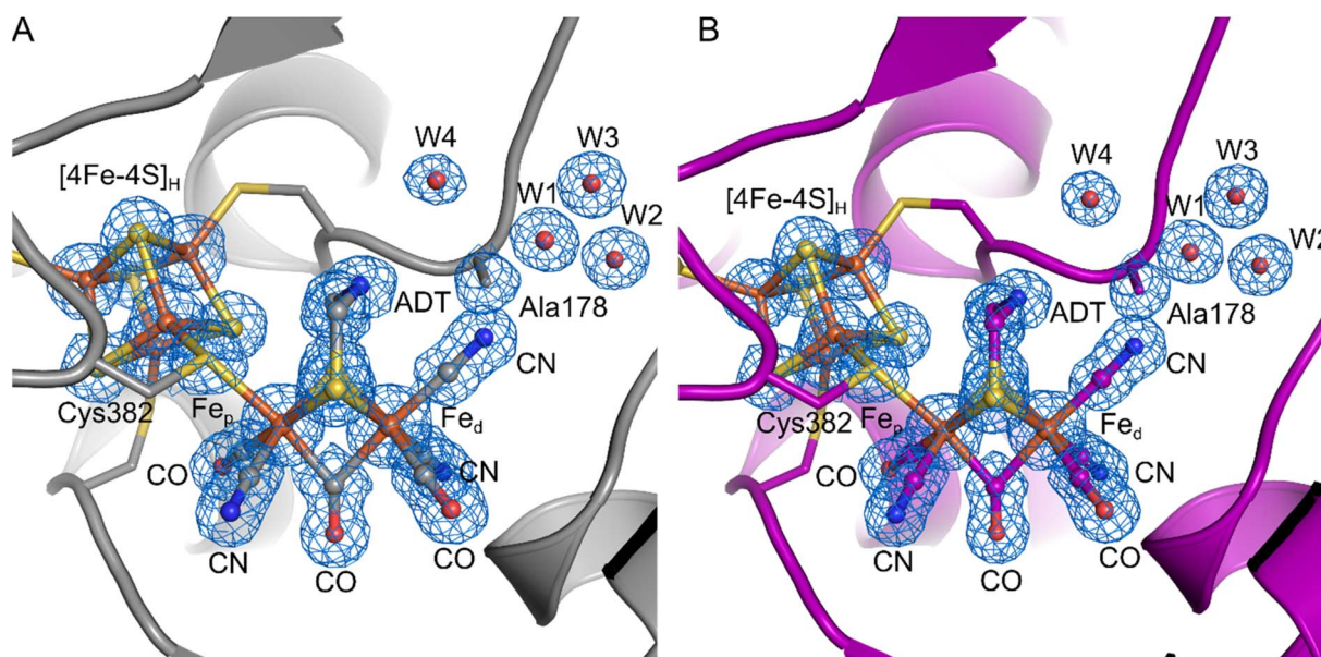
Fig. 4 Crystal structures of the DdHsdAB C178A mutant in two different states. (A) DdHsdAB in the \text{H}_{\text{inact}} -like state (PDB ID 8BJ7) is shown as cartoon and colored in gray. (B) DdHsdAB in the \text{H}_{\text{trans}} -like state (PDB ID 8BJ8) is shown as cartoon and colored in magenta. Close-up view of the active site showing the H-cluster, the Cys ligating the cofactor, the side chain of Ala178 and the well-defined water molecules with a distance <4.0 Å from Ala178. The protein backbone is shown as cartoon, the amino acid side chains and the H-cluster including the bound \text{CN}^- are shown as stick model, and water molecules are shown as spheres. The cofactors and amino acid side chains are colored according to the element-specific color code. A 2\text{Fo}-\text{Fc} electron density map (blue mesh, contoured at 1.0\sigma ) is shown for the H-cluster including the \text{CN}^- ligand, the side chain of Ala178, and the water molecules.
