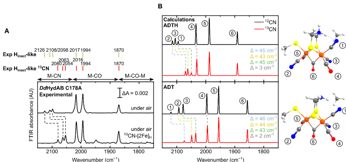
Fig. 3 (A) Experimental IR spectra of DdHsdAB C178A matured with natural abundance (top) and ^{13}\text{C}^- -labeled [2\text{Fe}]_{\text{H}} precursor (bottom), both exposed to air to form the \text{H}_{\text{inact}} -like state. The small additional feature in the ^{13}\text{C} spectrum may represent a small amount of an unknown degradation product. (B) Calculated IR spectra of the H-cluster model with either a singly protonated (ADT) or doubly protonated (ADTH) ADT ligand. Insets are [2\text{Fe}]_{\text{H}} structures with chemical groups associated with modes labelled. A scaling factor of 0.964 was used.
