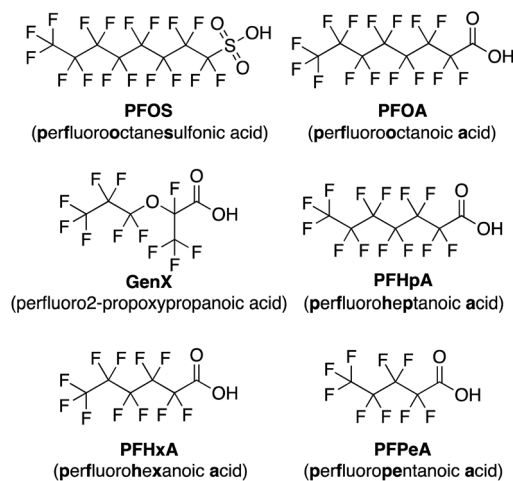
Fig. 2 Structures of the PFAS detected by the imprint-and-report array.
