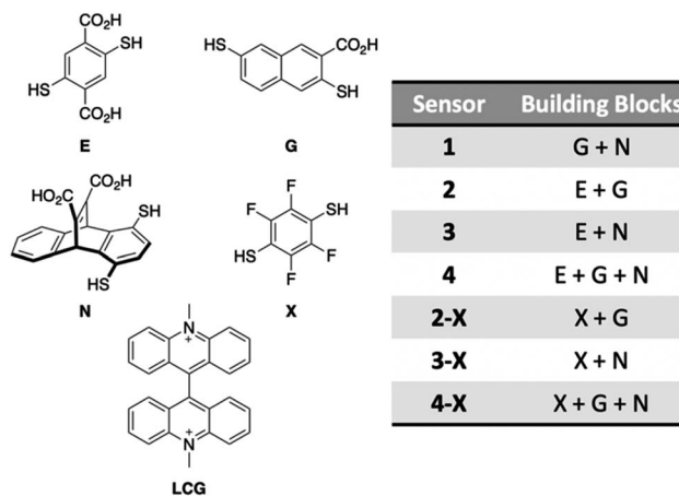
Fig. 3 Structures of DCC building blocks E, G, N, and X and the fluorophore template LCG (left), and the composition of each DCL sensor (right).
