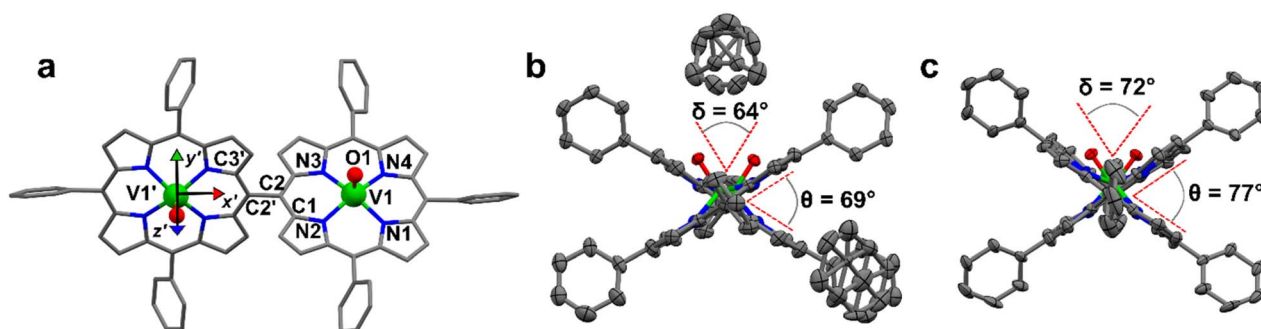
Fig. 1 (a) Molecular structure of [\text{VO}(\text{TrPP})]_2 with labeled atoms. The local xyz (not shown for clarity's sake) and x'y'z' reference frames are those diagonalizing \mathbf{g} - and \mathbf{A} -tensors of the two vanadyl moieties. Primed labels indicate atoms related to non-primed ones by the C_2 symmetry axis bisecting the m - m bond. (b and c) View along the m - m bond of the m\text{-}[\text{VO}(\text{TrPP})]_2 and o\text{-}[\text{VO}(\text{TrPP})]_2 molecules. The dihedral angle, \theta , between the porphyrin planes and the torsion angle, \delta , between the vanadyl moieties' directions are highlighted by red dashed lines; atoms in (b and c) are represented as thermal ellipsoids at 50% probability level. Color code: C = gray; N = blue; V = green; O = red. Only the majority configuration of the V=O groups is reported. H-atoms are omitted for clarity.
