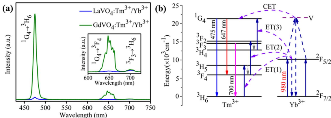
Fig. 3 (a) Comparison of upconversion emission spectra of 0.3 mol% \text{Tm}^{3+} /5 mol% \text{Yb}^{3+} codoped \text{LaVO}_4 and \text{GdVO}_4 phosphors under 980 nm laser diode excitation; inset shows the enlarged spectra in 600–730 nm range; (b) energy level diagram of \text{Tm}^{3+} and \text{Yb}^{3+} ions with possible upconversion processes in both the hosts.
