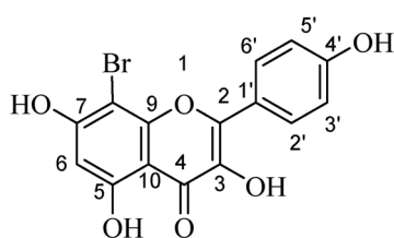
Fig. 1 Chemical structures of isolated compounds.
