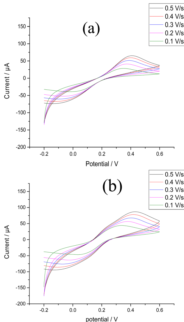
Fig. 5 CV results for 1.0 mM K_4[Fe(CN)_6] in 0.1 M KCl using scan rates of 0.1–0.5 V s -1 at (a) the bare CPE (b) the Bi–Sb/CPE.
