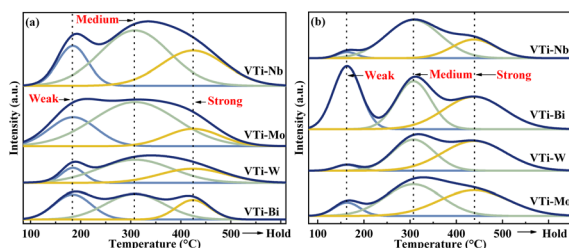
Fig. 6 \text{NH}_3 - and \text{CO}_2 -TPD profiles of metal cation-doped VPO catalysts: (a) \text{NH}_3 -TPD, (b) \text{CO}_2 -TPD.
