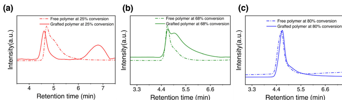
Fig. 4 SEC traces for free polymers from solution (FP) and grafted polymers (GP) from polystyrene grafted silica synthesized via ESCP (PSRHA) at (a) 25% conversion, (b) 68% conversion, and (c) 80% conversion. The free polymers were obtained by precipitating the decant in cold methanol after centrifugation and the grafted polymers were cleaved by transesterification of polystyrene grafted silica synthesized via ESCP using p -toluenesulfonic acid and methanol in toluene. The broader dispersity and multiple populations of grafted polystyrene than that of the single population of free polymers was observed due to the ability of surface nitrene functionalities to capture and terminate the growing polymer radicals at any stage of propagation. The molecular weight of grafted polystyrene observed at 25% conversion was 85\,000\text{ g mol}^{-1} , with respect to the 38\,000\text{ g mol}^{-1} of free polymers, which confirms the potential of nitrene functionalities to capture two polymer radicals.
